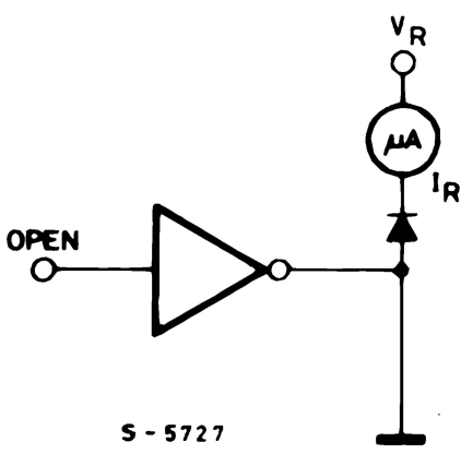
Figure 9. Clamp diode leakage current
