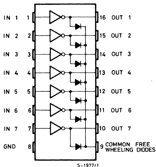
Figure 2. Pin connections (top view)
