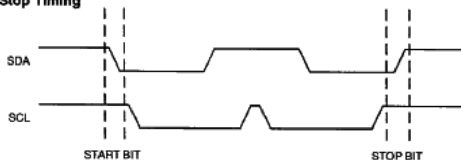
Figure 3. Start/Stop Timing
