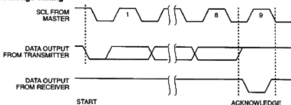
Figure 4. Acknowledge Timing
