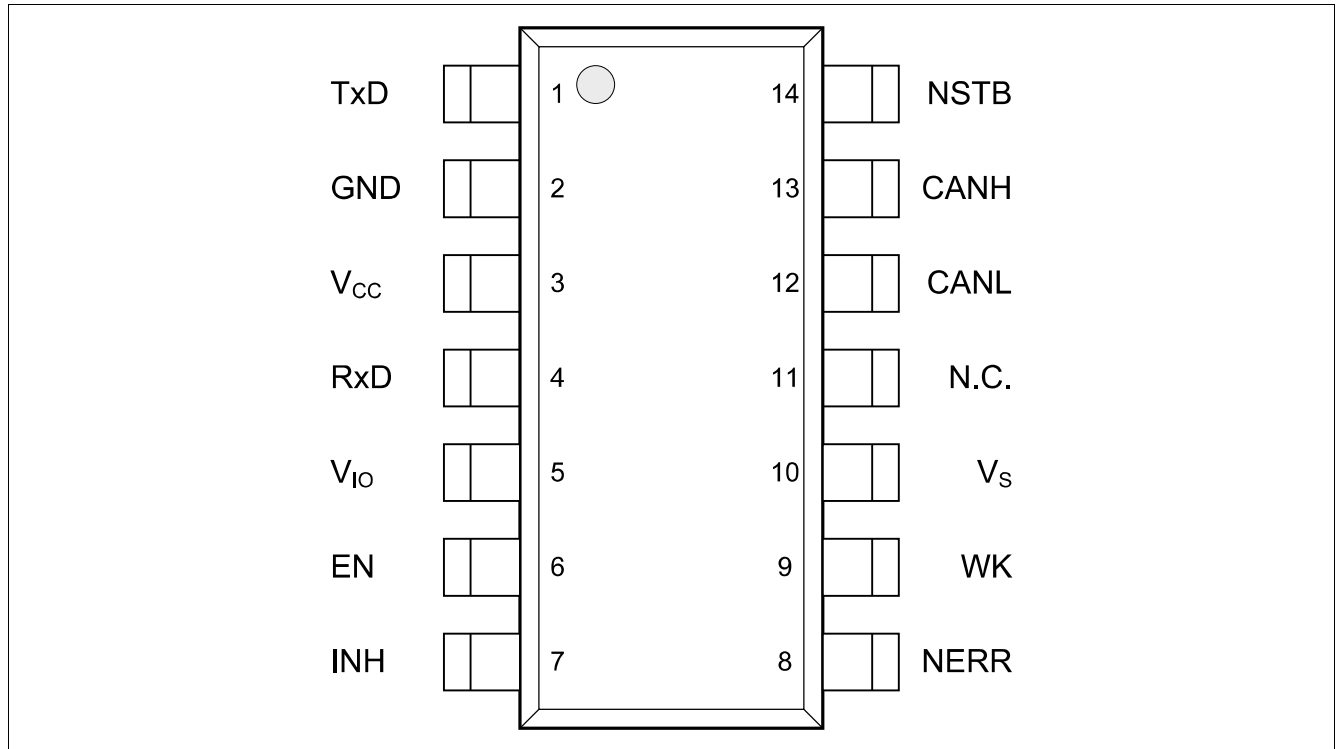
Figure 2 Pin Configuration
