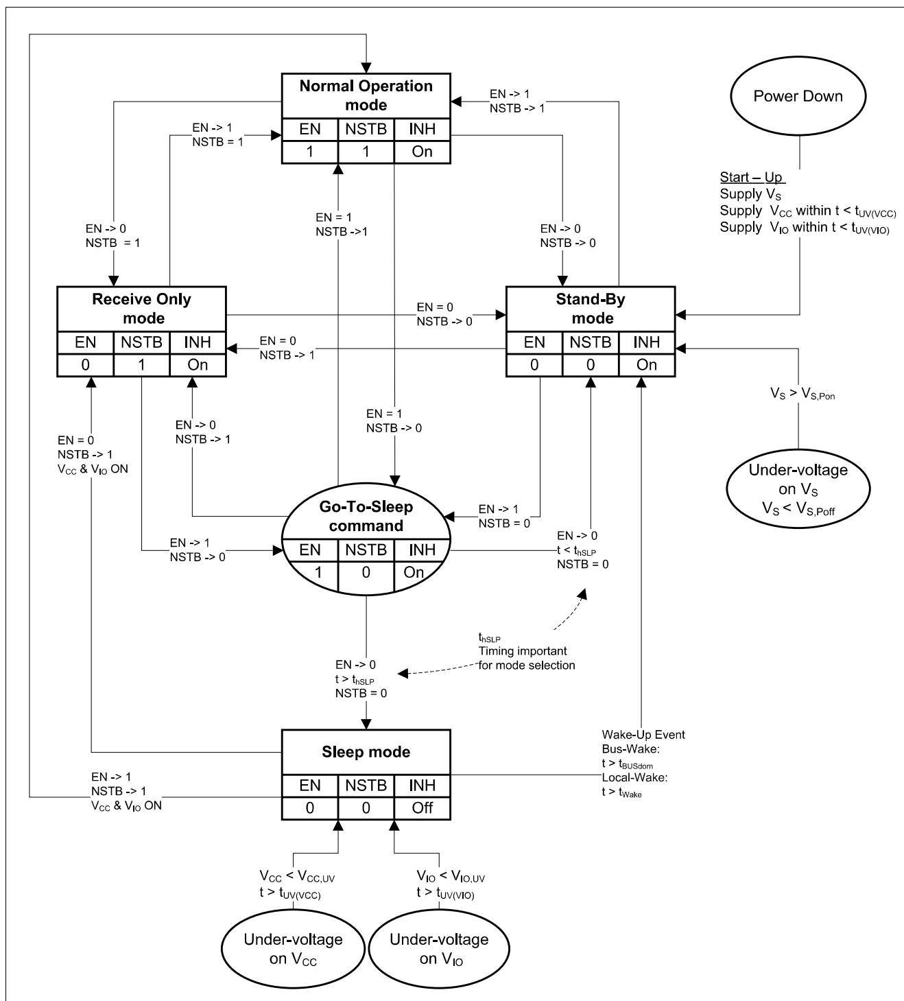
Figure 4 Operation Modes
