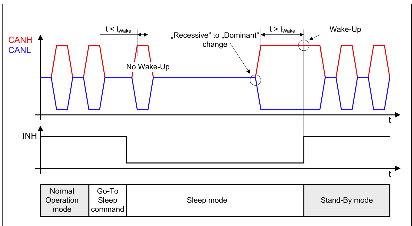
Figure 6 Remote Wake-Up
