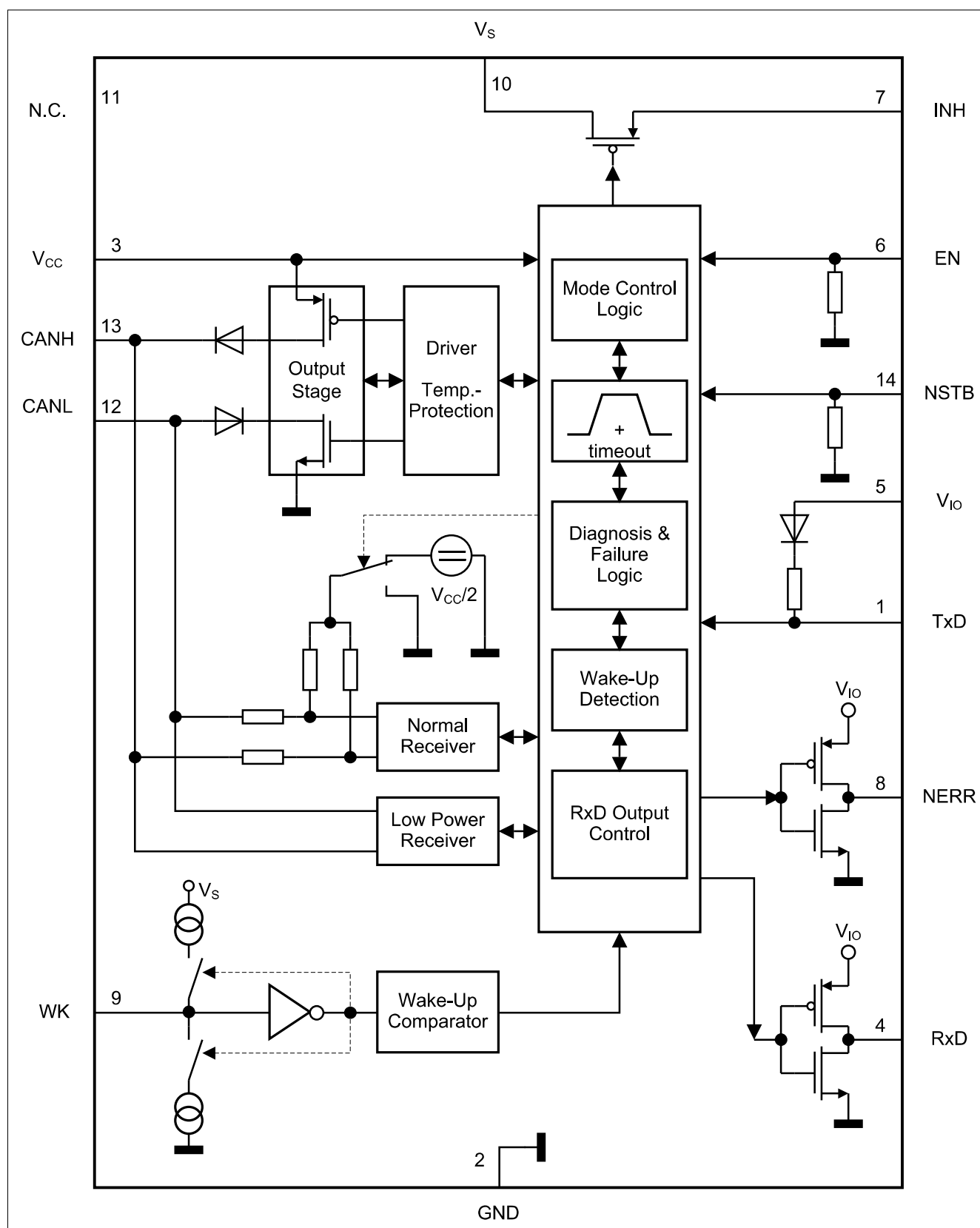
Figure 1 Block Diagram
