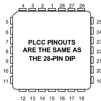
28-Pin PLCC 73K222AL-IH
