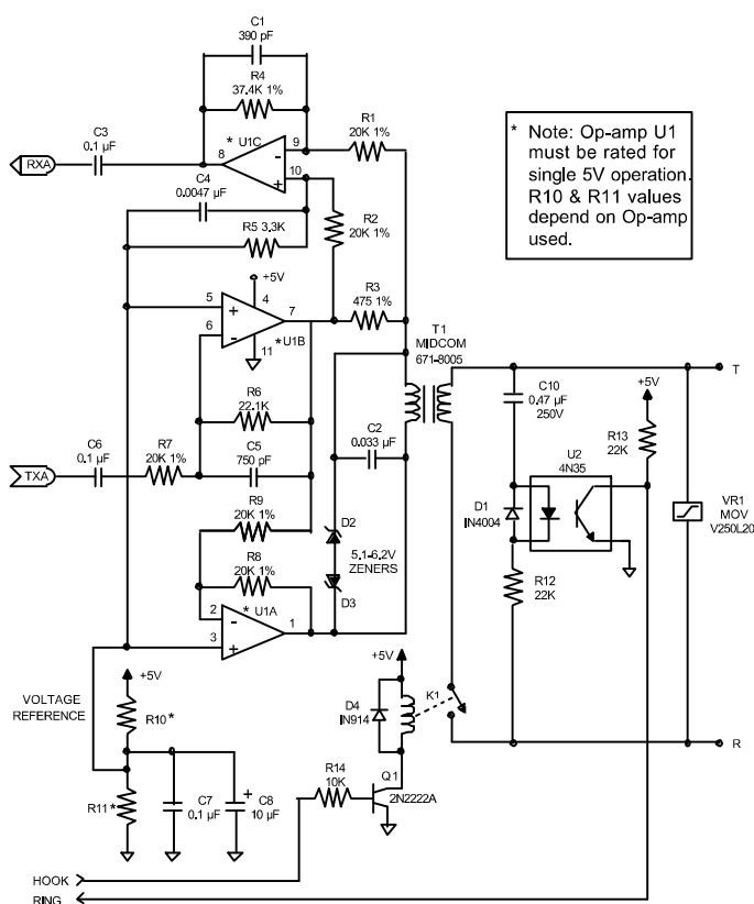
FIGURE 2: Single 5V Hybrid Version
