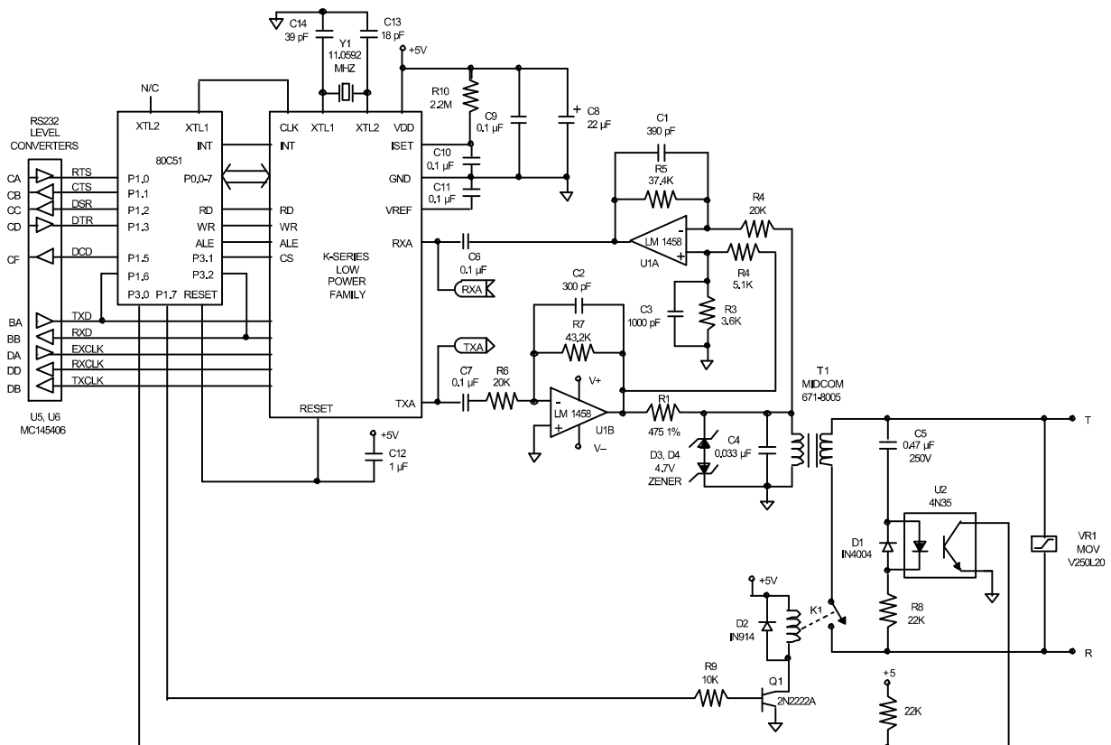
FIGURE 1: Basic Box Modem with Dual-Supply Hybrid
