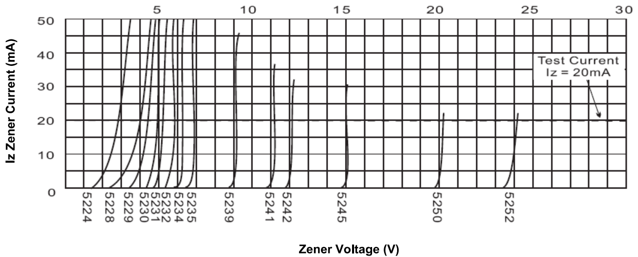
Fig.2 Breakdown Characteristics
