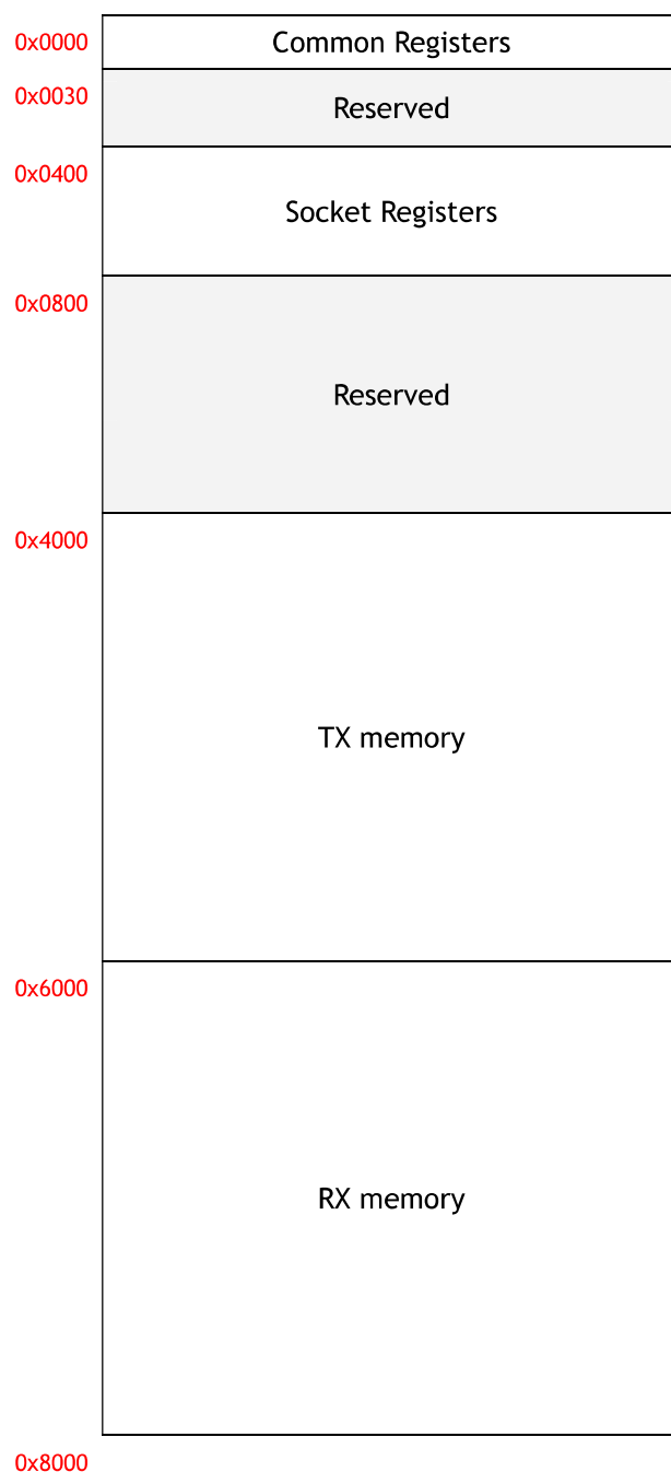
Memory Map
