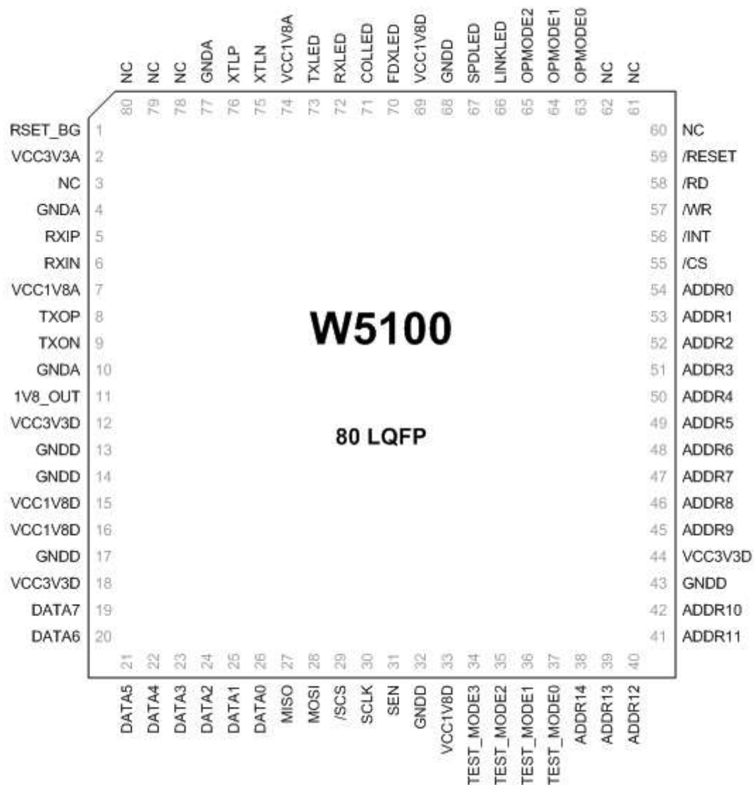
Pinout W5100
