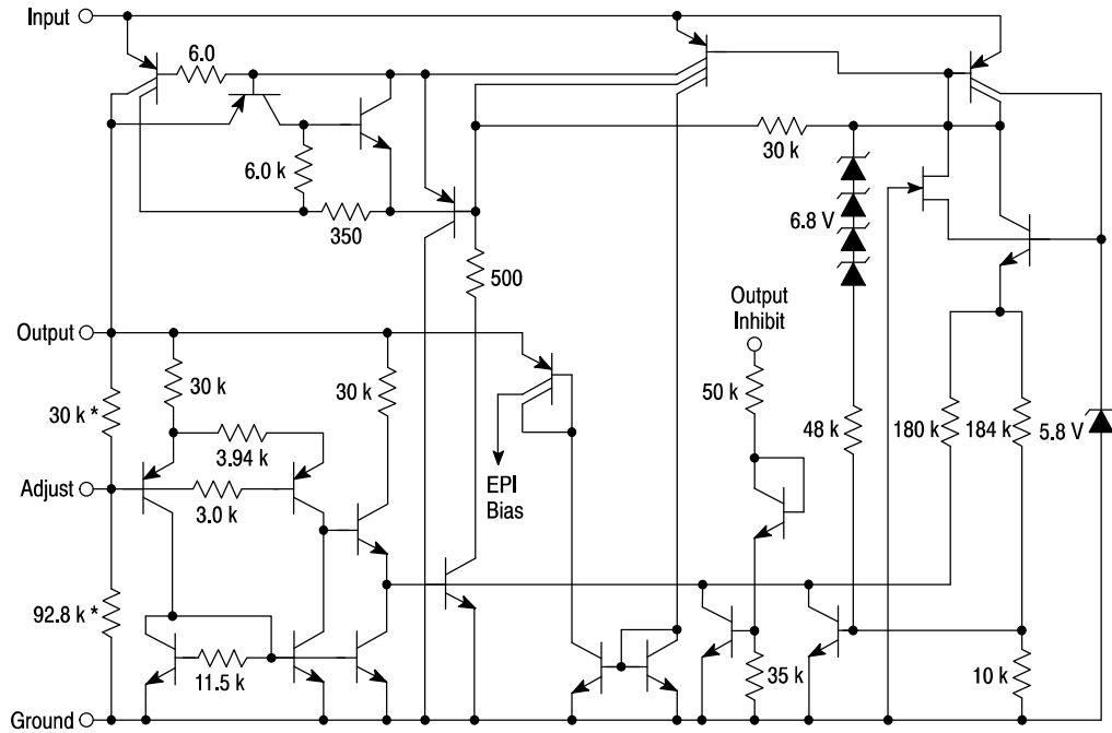
Figure 1. Representative Schematic Diagram
