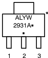
SOT-223 ST SUFFIX CASE 318H
