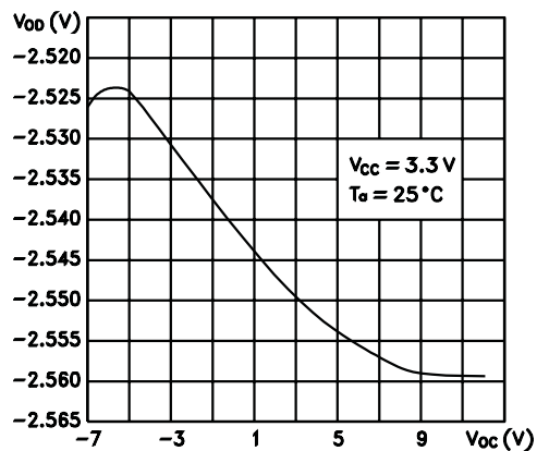
Figure 22. Low level driver output capability
