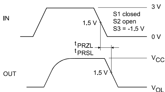
Figure 18. Receiver enable and disable times waveform (test 3)
