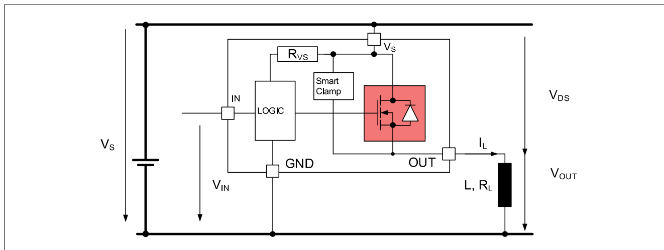
Figure 9 Output Clamp
