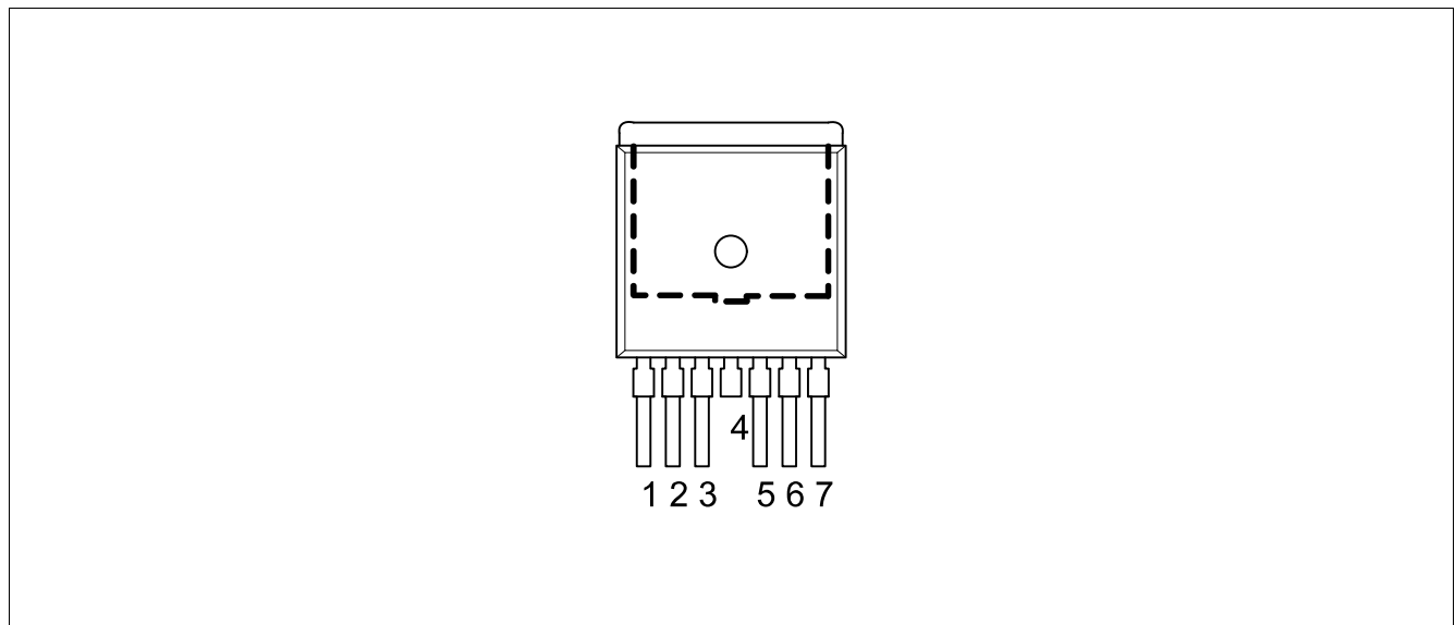
Figure 2 Pin Configuration
