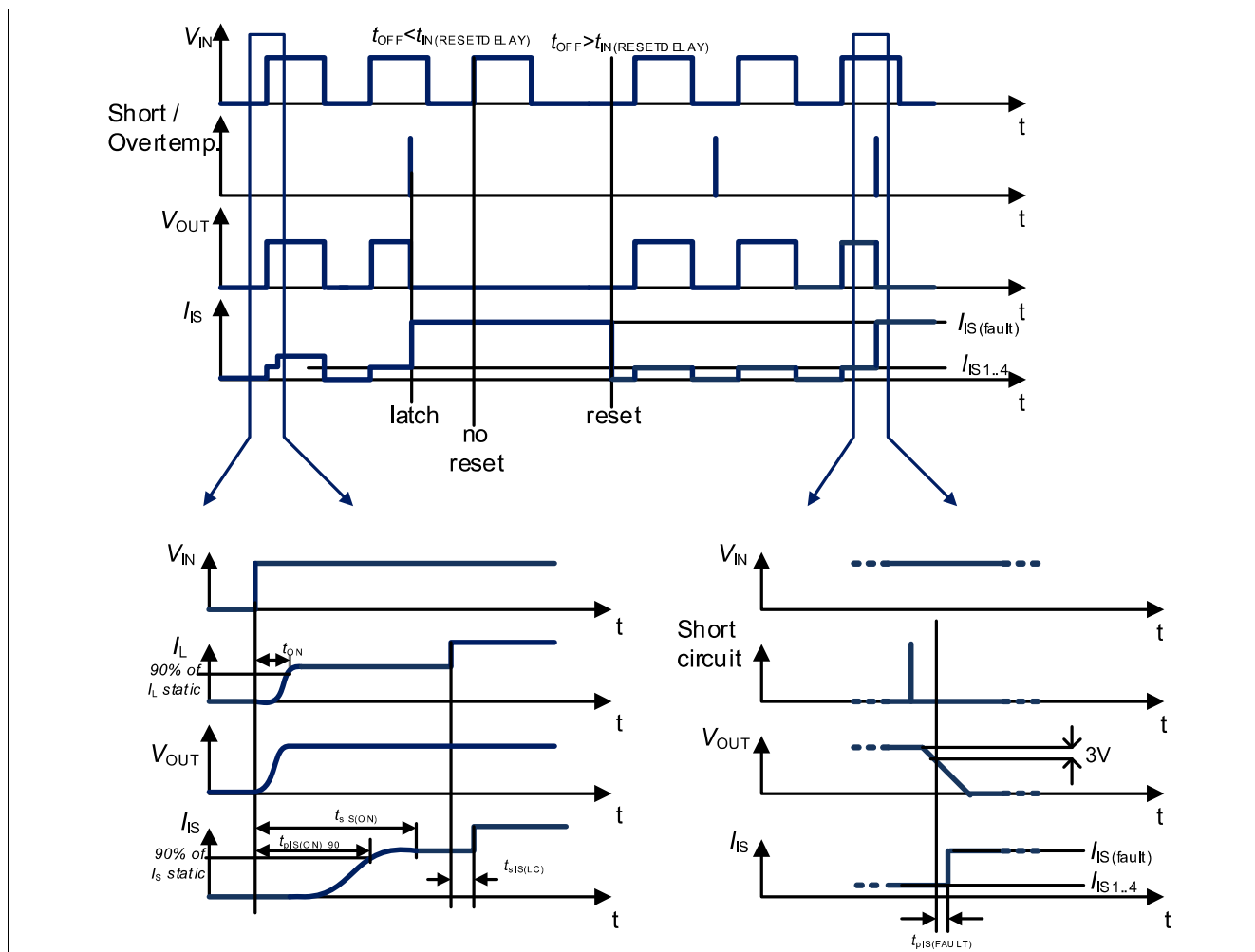
Figure 30 Fault Acknowledgement
