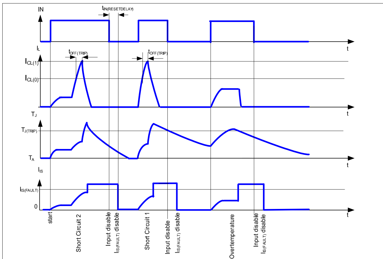
Figure 26 Overload Protection
