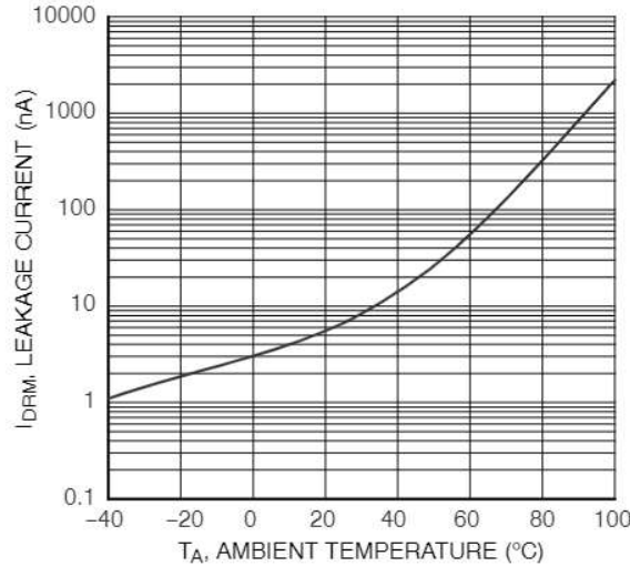
Figure 4. Leakage Current, I_{DRM} vs. Temperature
