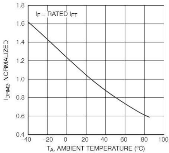
Figure 5. I_{DRM2} - Leakage in Inhibit State vs. Temperature
