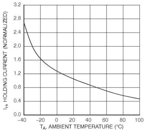
Figure 7. Holding Current, I_H vs. Temperature
