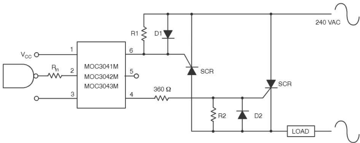
Figure 12. Inverse-Parallel SCR Driver Circuit (MOC3041M, MOC3042M, MOC3043M)
