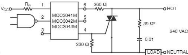
Figure 10. Hot-Line Switching Application Circuit (MOC3041M, MOC3042M, MOC3043M)
