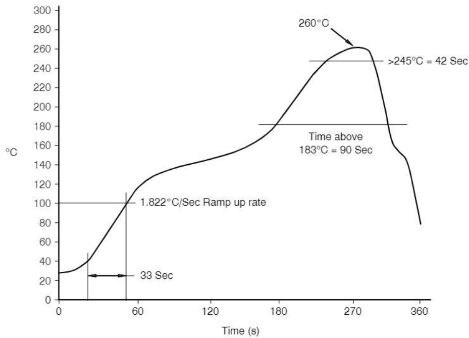
Figure 13. Reflow Profile
