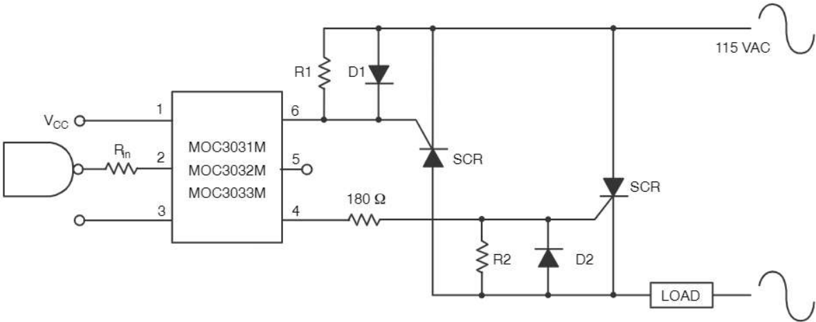
Figure 11. Inverse-Parallel SCR Driver Circuit (MOC3031M, MOC3032M, MOC3033M)
