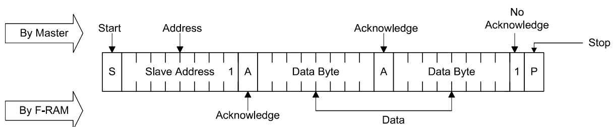
Figure 10. Sequential Read
