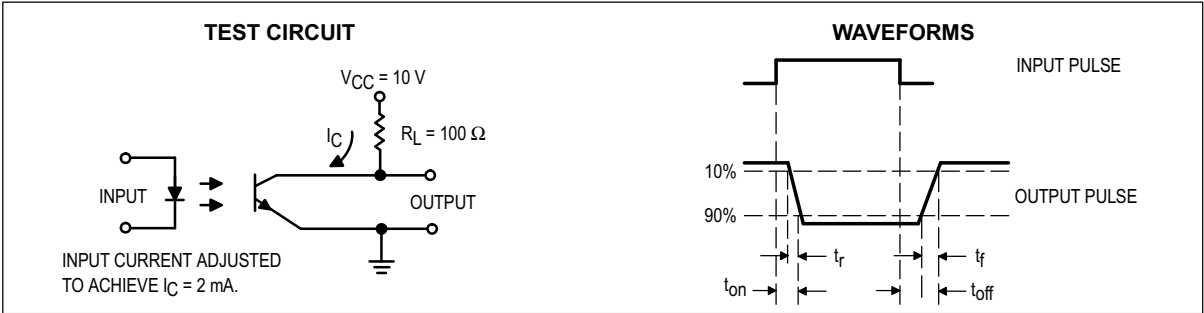
Figure 10. Switching Time Test Circuit and Waveforms
