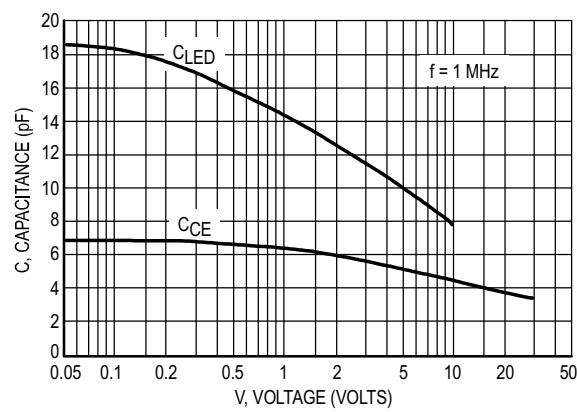
Figure 9. Capacitances versus Voltage
