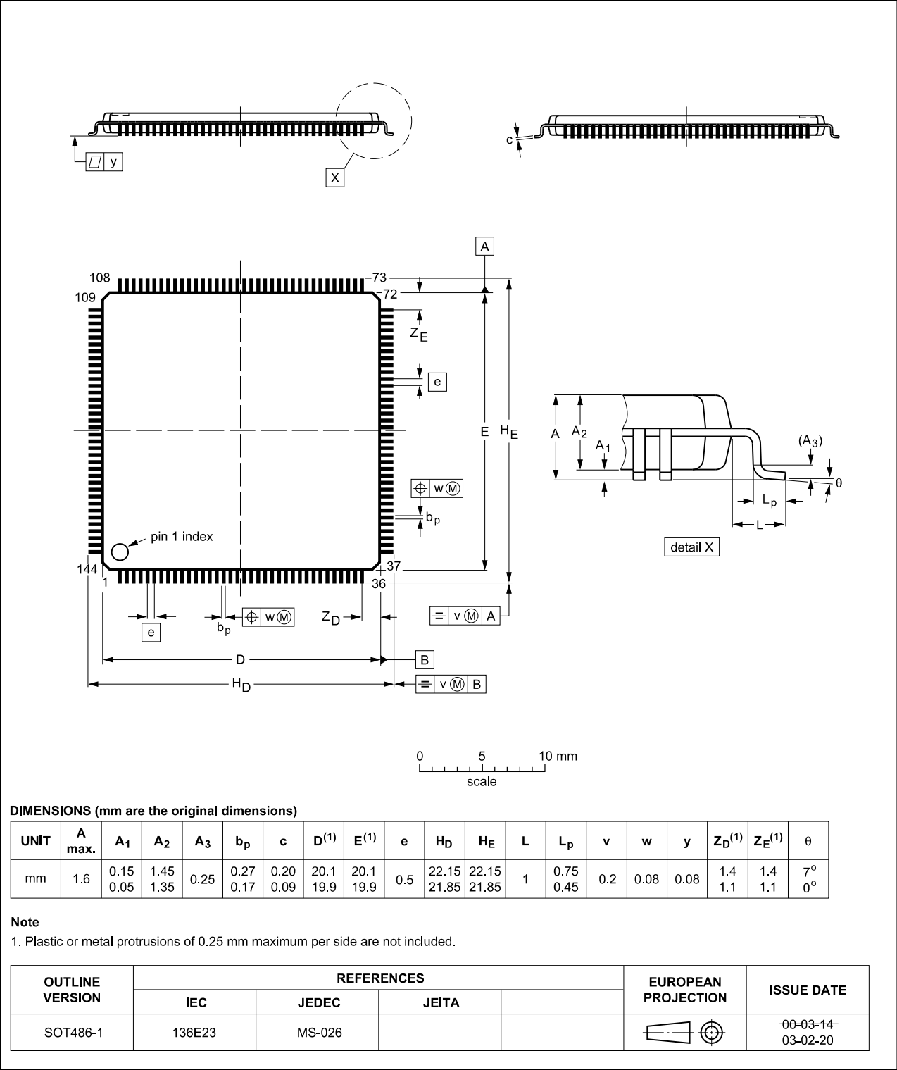
Fig 44. LQFP144 package
