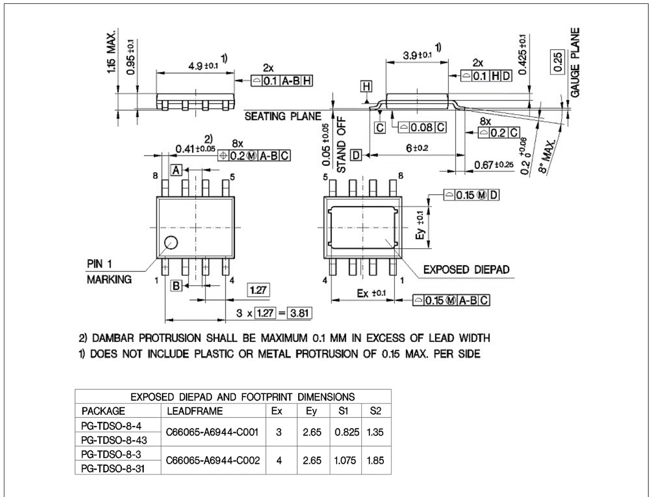
Figure 47 PG-TDSO8-31
