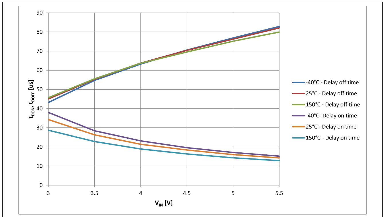
Figure 27 Typical t_{DON} , t_{DOFF} vs V_{IN} @ T_J = -40 \dots 150^\circ C
