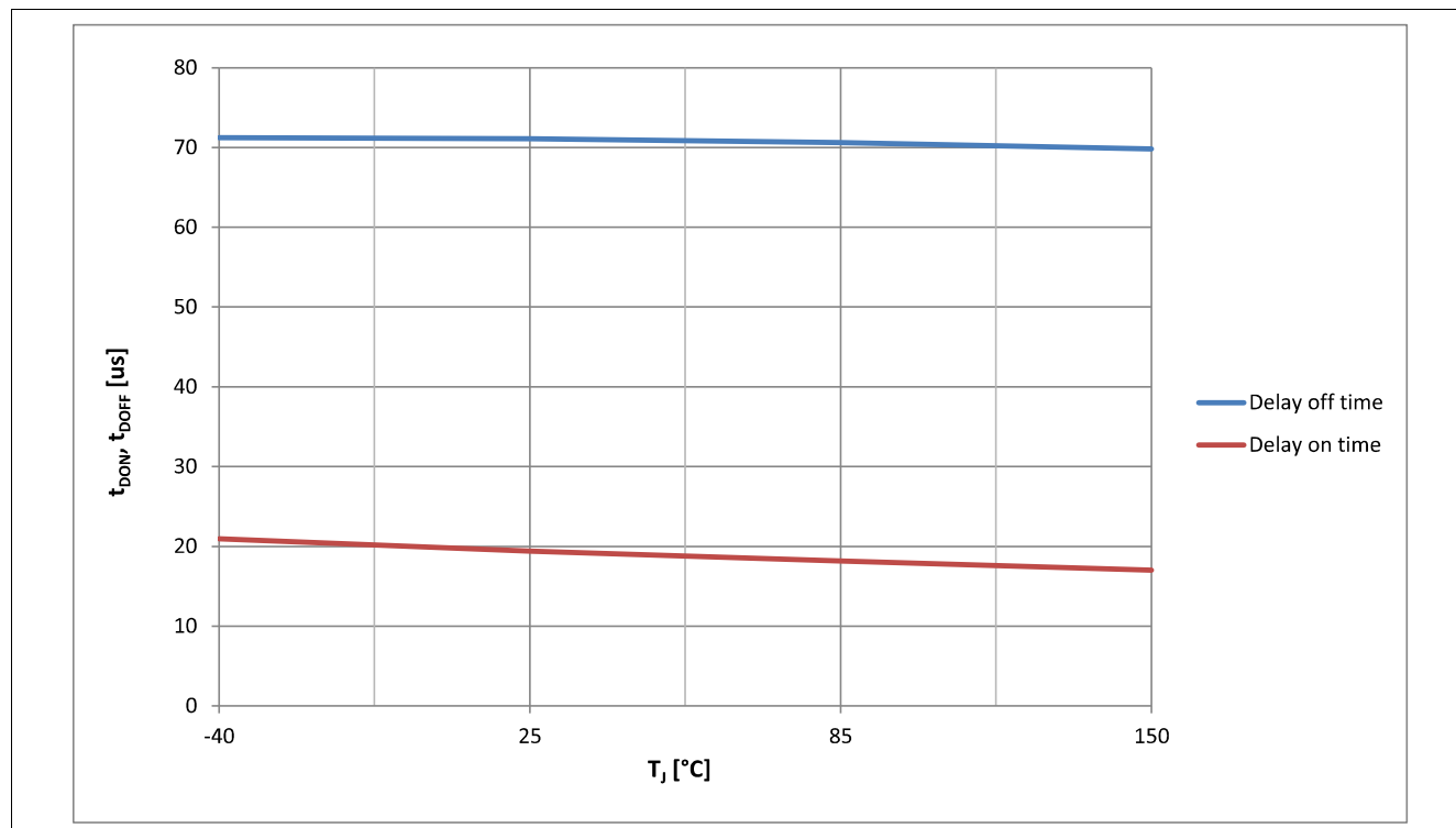
Figure 36 Typical t_{ON} , t_{OFF} vs T_J @ V_{IN} = 5 V
