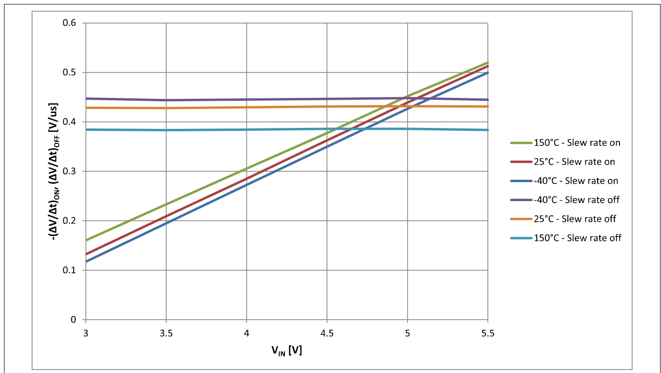
Figure 28 Typical -(\Delta V/\Delta t)_{ON} , (\Delta V/\Delta t)_{OFF} vs V_{IN} @ T_J = -40 \dots 150^\circ C
