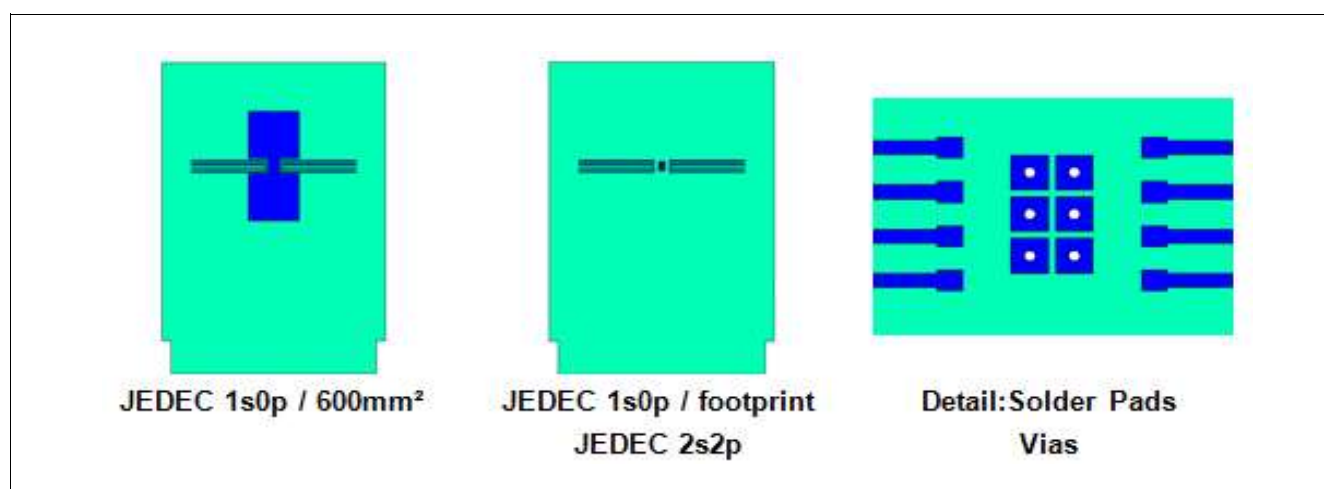
Figure 6 PCB layout
