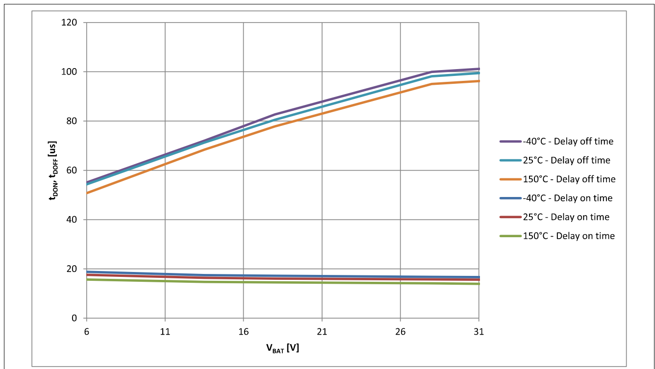
Figure 30 Typical t_{ON} , t_{OFF} vs V_{BAT} @ V_{IN} = 5\text{ V} , T_J = -40 \dots 150^\circ\text{C}
