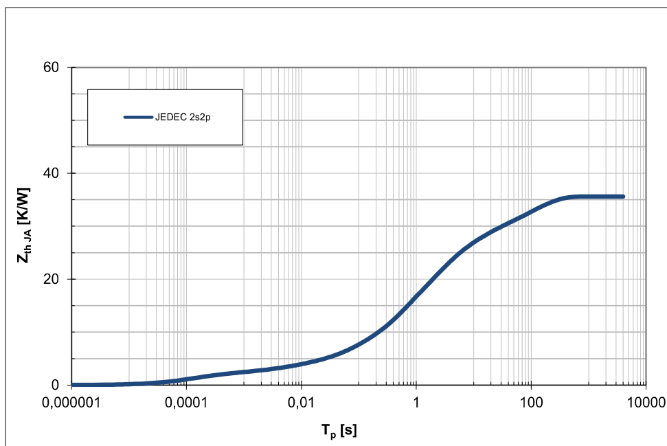
Figure 7 Typical transient thermal impedance Z_{thJA} = f(t_p) , T_A = 85^\circ\text{C} Value is according to Jedec JESD51-2,-7 at natural convection on FR4 2s2p board; The product (Chip + Package) was simulated on a 76.2 \times 114.3 \times 1.5 \text{ mm}^3 board with 2 inner copper layers (2 x 70 \mu\text{m} Cu, 2 x 35 \mu\text{m} Cu). Device is dissipating 1 W power.
