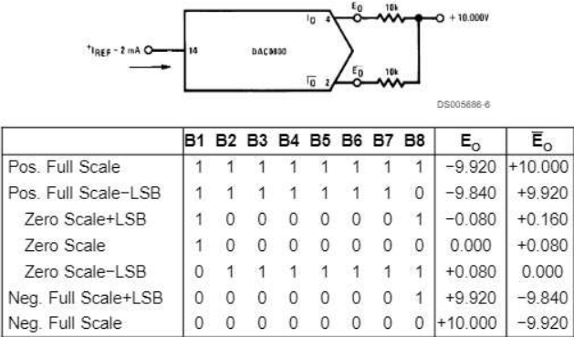
FIGURE 7. Basic Bipolar Output Operation (Note 5)
