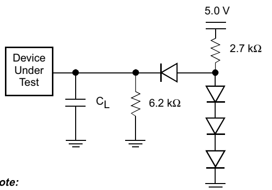
Figure 3. Test Setup
