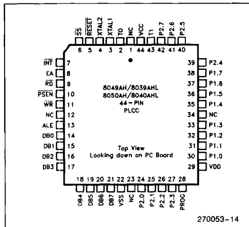
Figure 4. Pad Configuration
