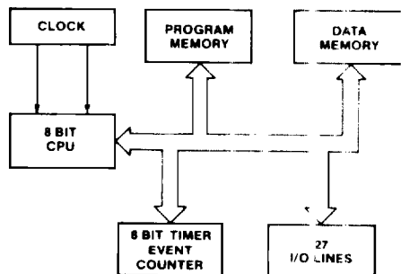
Figure 1. Block Diagram
