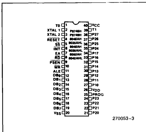
Figure 3. Pin Configuration
