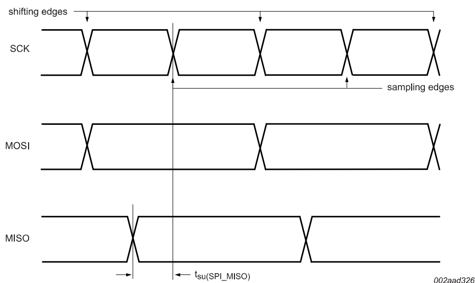
Fig 14. MISO line set-up time in SSP Master mode
