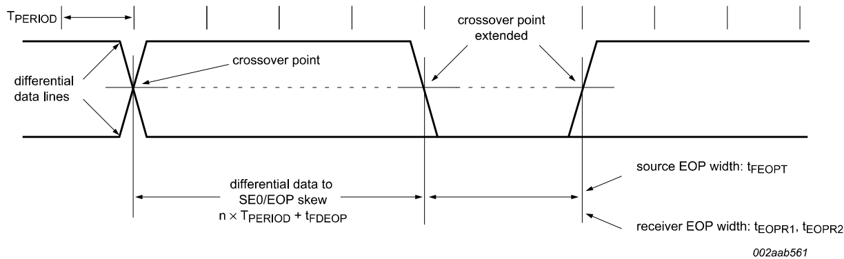
Fig 13. Differential data-to-EOP transition skew and EOP width
