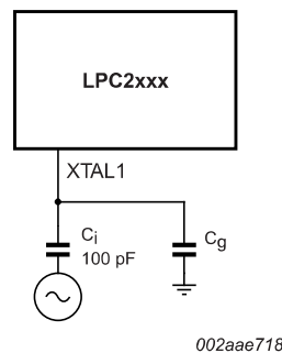
Fig 22. Slave mode operation of the on-chip oscillator
