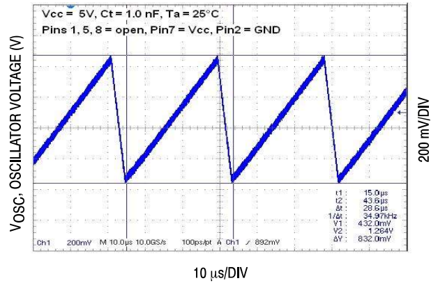
Figure 4. Timing Capacitor Waveform
