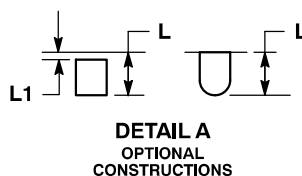
DFN8, 4x4 CASE 488AF-01 ISSUE C
