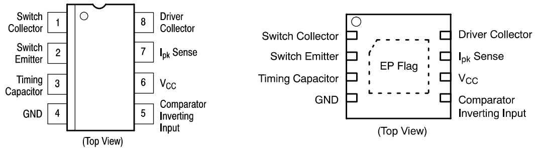
Figure 2. Pin Connections
