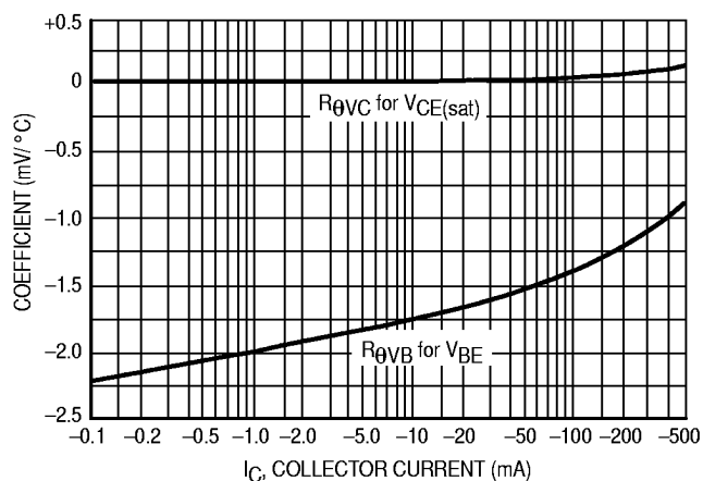
Figure 12. Temperature Coefficients
