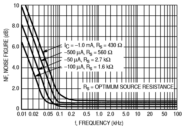
Figure 7. Frequency Effects
