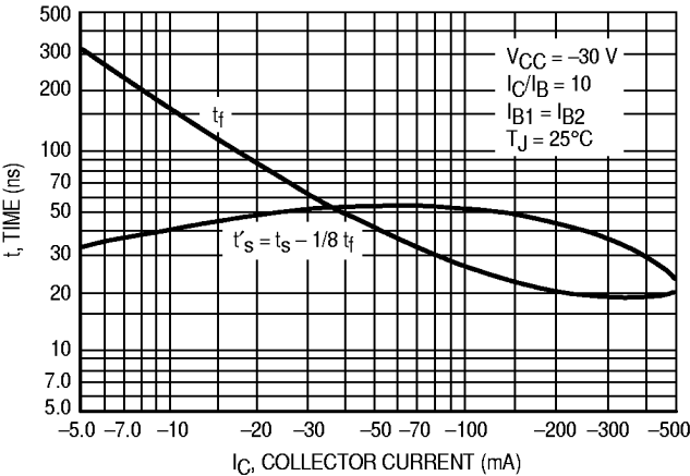
Figure 6. Turn-Off Time
