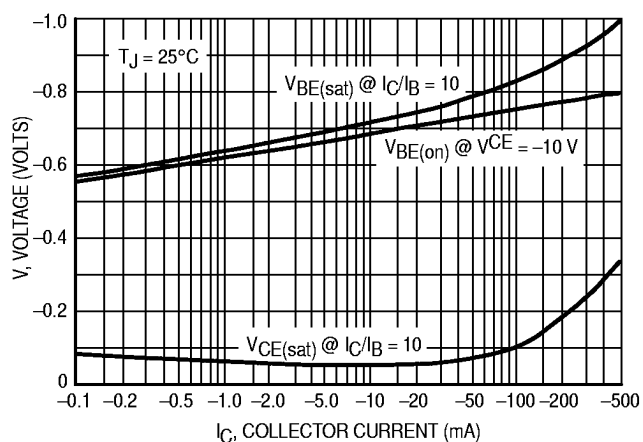
Figure 11. "On" Voltage
