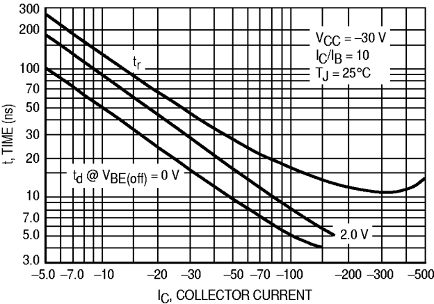
Figure 5. Turn-On Time
