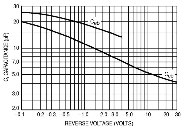
Figure 9. Capacitances
